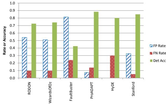
Figure 13: ADAPT false positive rate, false negative rate, and detection accuracy by DA.
