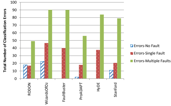
Figure 17: ADAPT classification errors per number of faults by DA.
