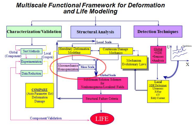
Figure 6. Multiscale framework describing the interaction between experimentation, analysis and detection techniques to enable accurate deformation and life modeling.
