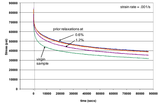
Figure 17. Stress-time results for relaxation at 1.8% strain from relaxation and step relaxation tests conducted at 427° C to demonstrate history dependence of viscoplastic behavior.
