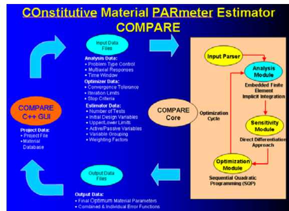
Figure 8. Flow chart for COMPARE software.
