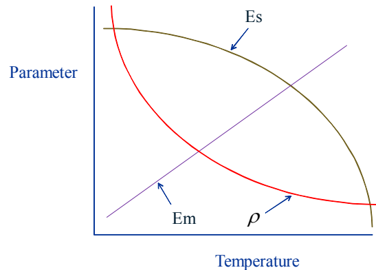
Figure 11. Variation of viscoelastic parameters with temperature.
