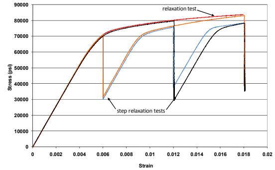
Figure 16. Stress-strain results from relaxation and step relaxation tests conducted at 427° C to demonstrate history dependence of viscoplastic behavior.
