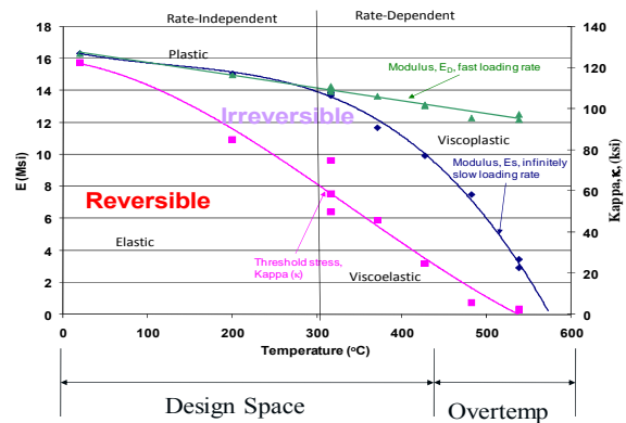
Figure 9 Variation of modulus and threshold stress as a function of temperature for Ti-6-4 material.
