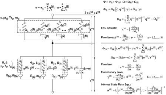
Figure 7. Analog representation of multi-mechanism deformation and damage GVIPS framework with key governing equations.
